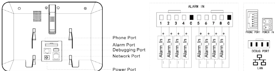
Rear panel of VTH1560B
