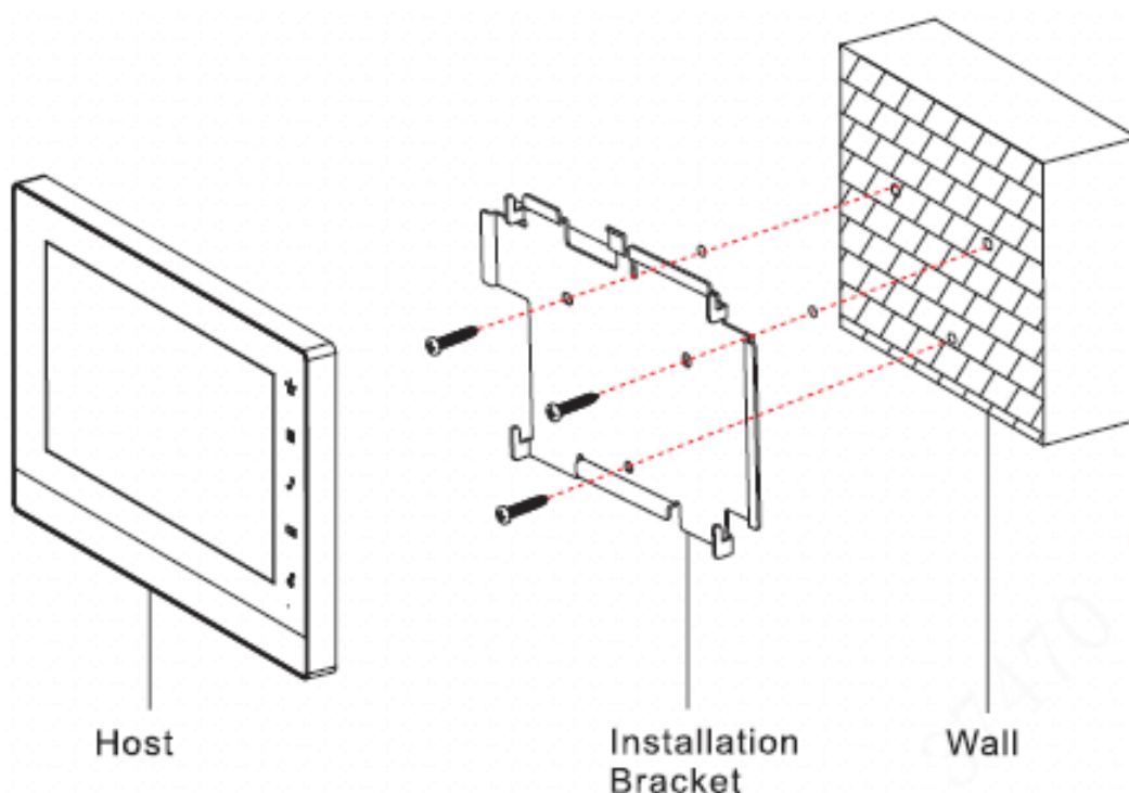
Figure 2-1 Wall-mounted installation
