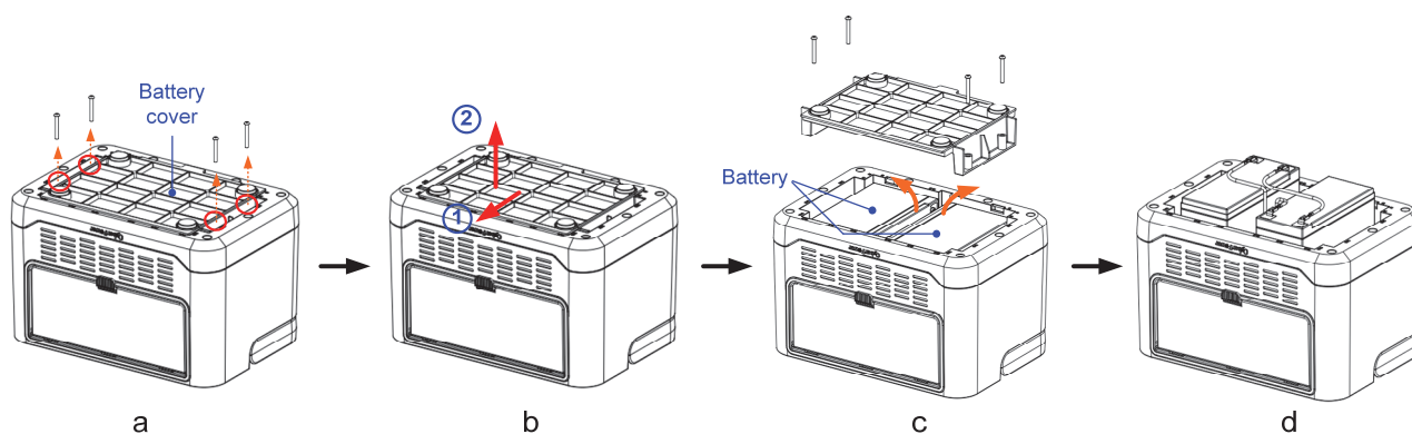
Fig. 8-1 Procedure of replacing batteries
