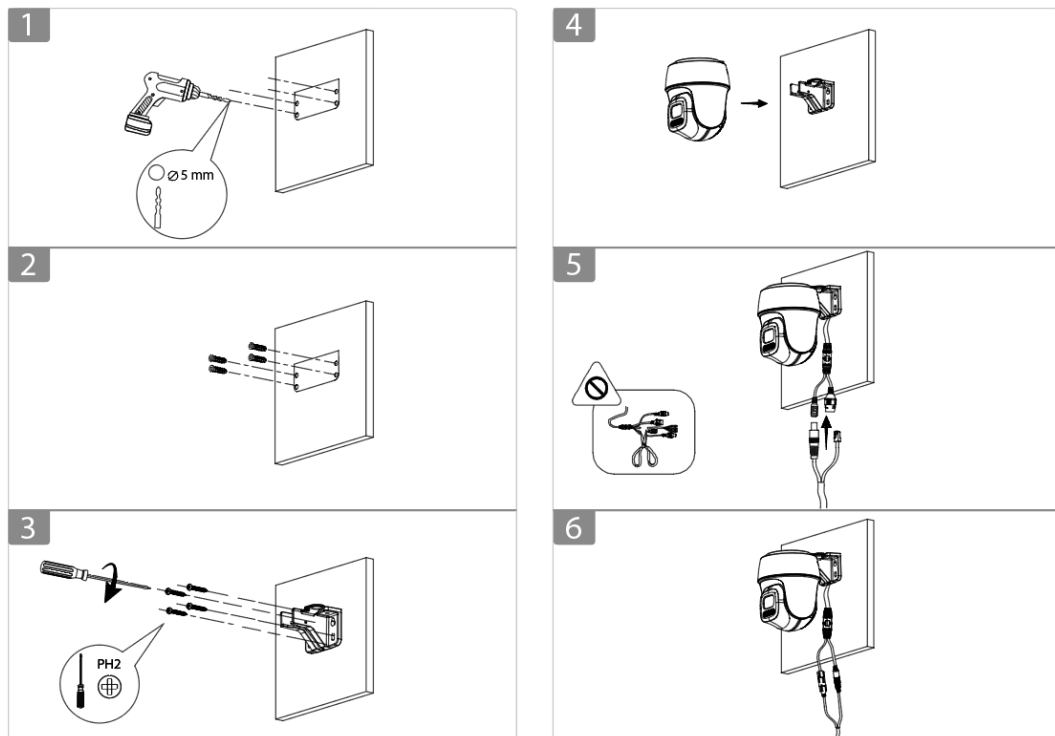
Figure 3-4 Wall mount
