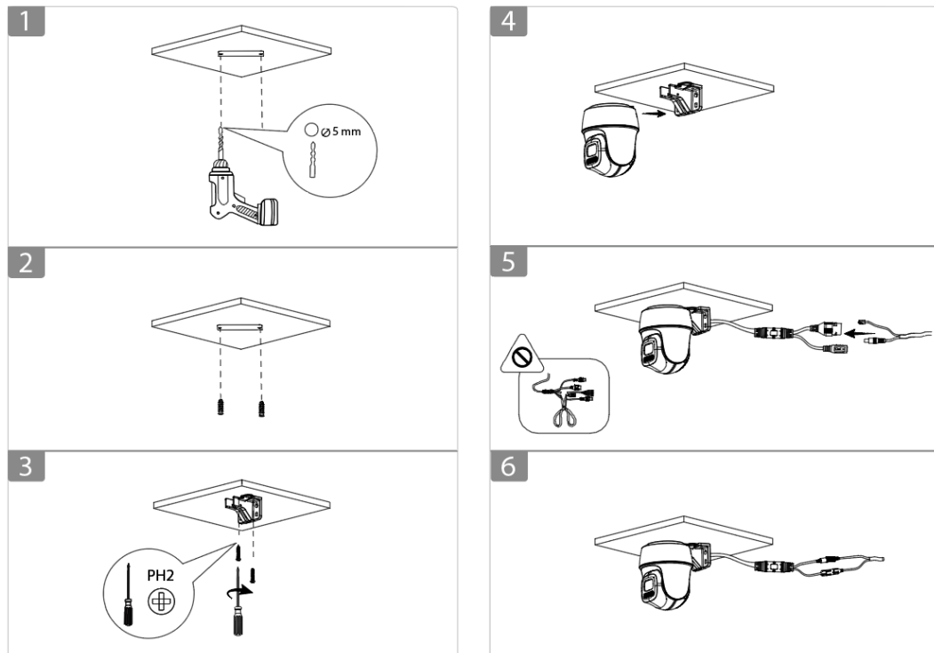
Figure 3-5 Ceiling mount
