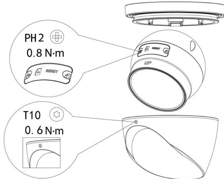
Figure 3-3 Install the SD card
