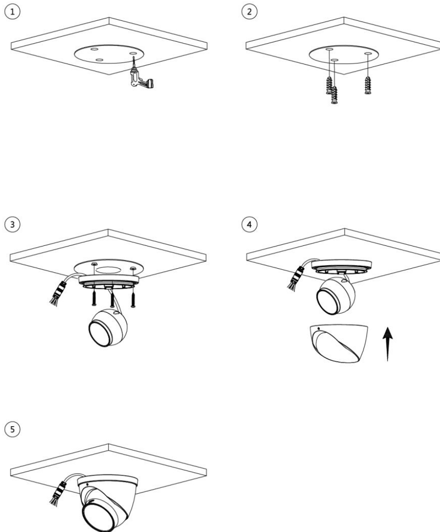
Figure 3-5 Cable going through the side cable tray
