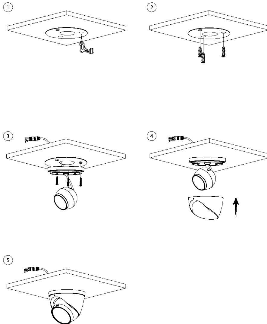
Figure 3-4 Cable going through the mounting surface
